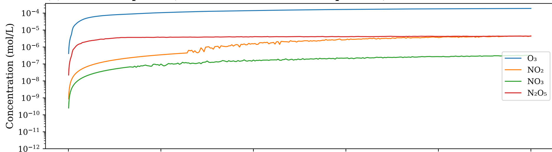
(c) RH 80% fitted + unmeasured (Dry)
