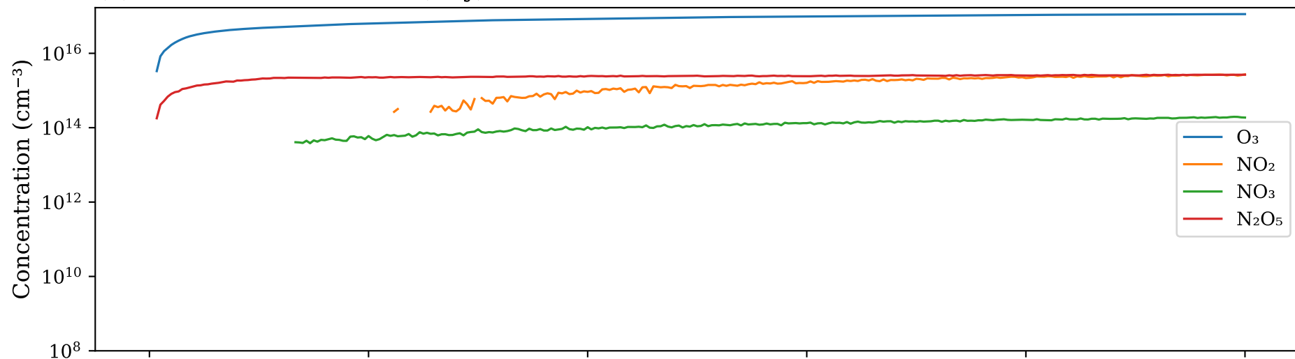
(b) Measured species (onset-filtered + linear interpolation)
