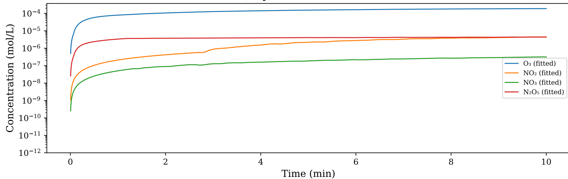
(c) RH 80% fitted + unmeasured (Dry)
